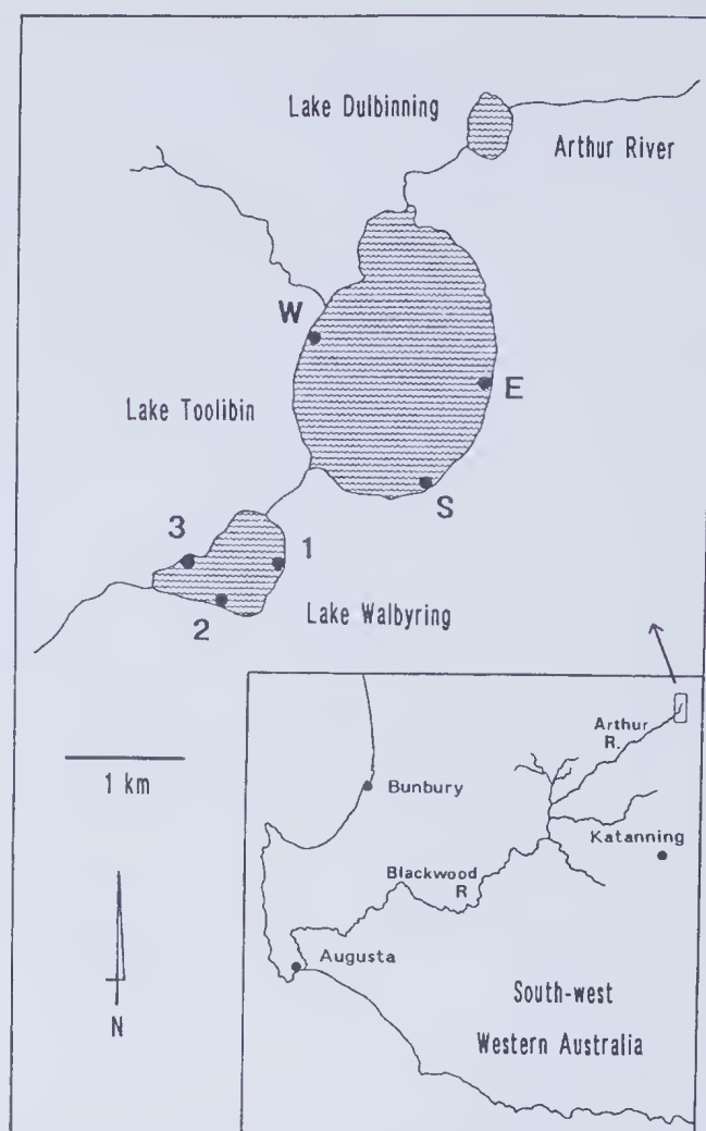
Figure 1. Sectors sampled for invertebrates at Toolibin and Walbyring Lakes on the Northern Arthur River, south-western Australia, and connection of the lakes with the Blackwood River.
